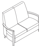
Open Arm Loveseat W57" D31" H43" Seat: W52" D19" H18" Arm Height: 28"
